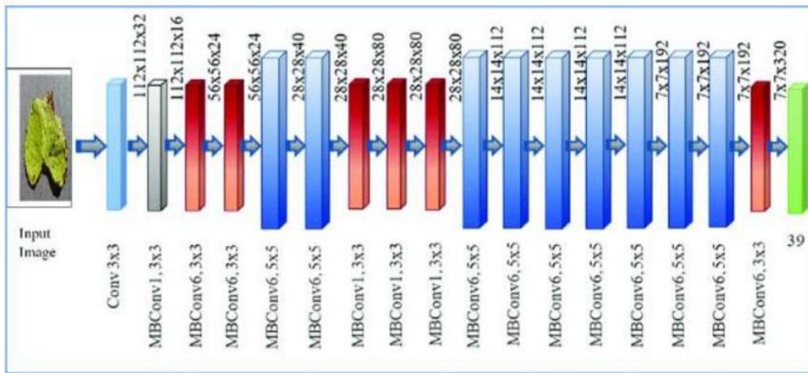
Fig 5: Architecture of EfficientNetB7.
