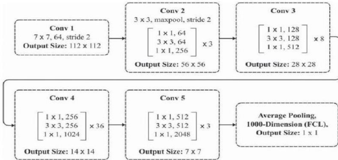
Fig 4: Architecture of ResNet152.
