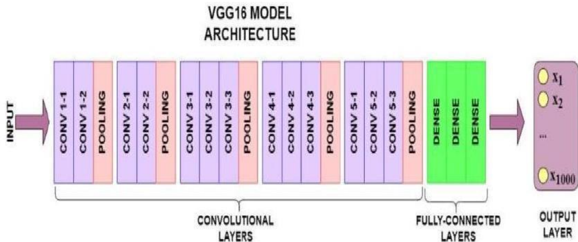
Fig 3: Architecture of VGG16
