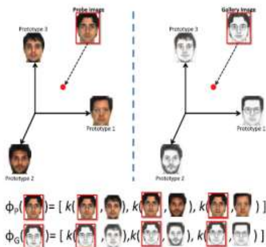
Fig: 1. Kernel Prototype based approach as a vector of their similarity to a set of common prototypes [01].
